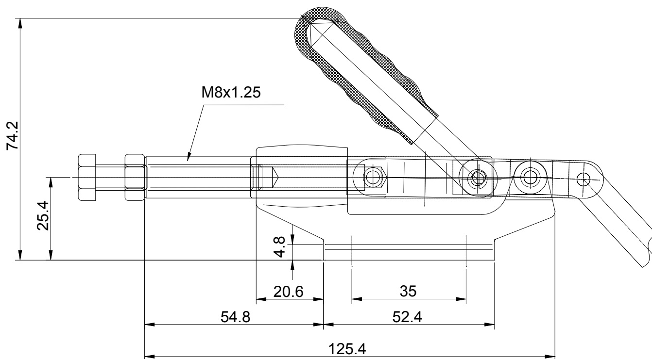
PLUNGER STORKE 32mm
